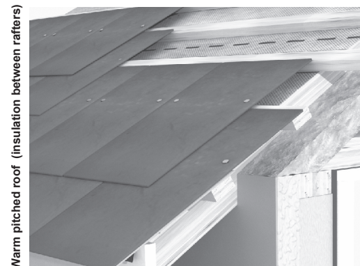
Habitable roof space (hybrid)
